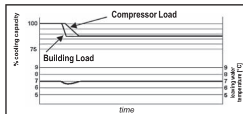
EWLT fluctuation with stepless capacity control
