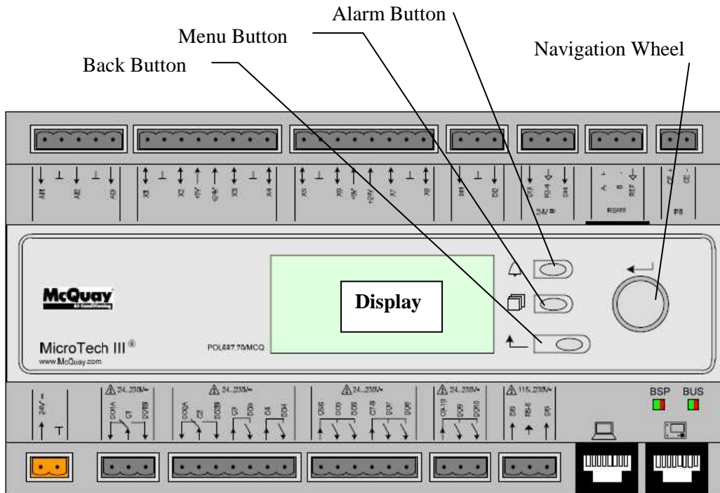
Figure 7, Unit Controller
